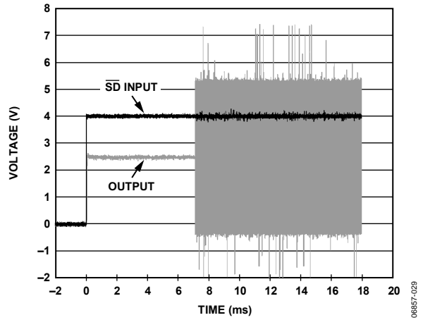
Figure 29. Turn-On Response
